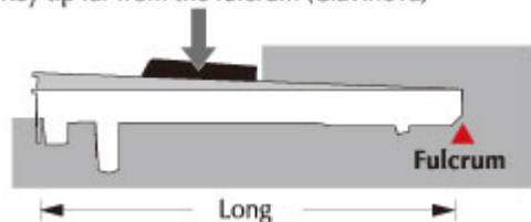
Key tip far from the fulcrum (Clavinova)
